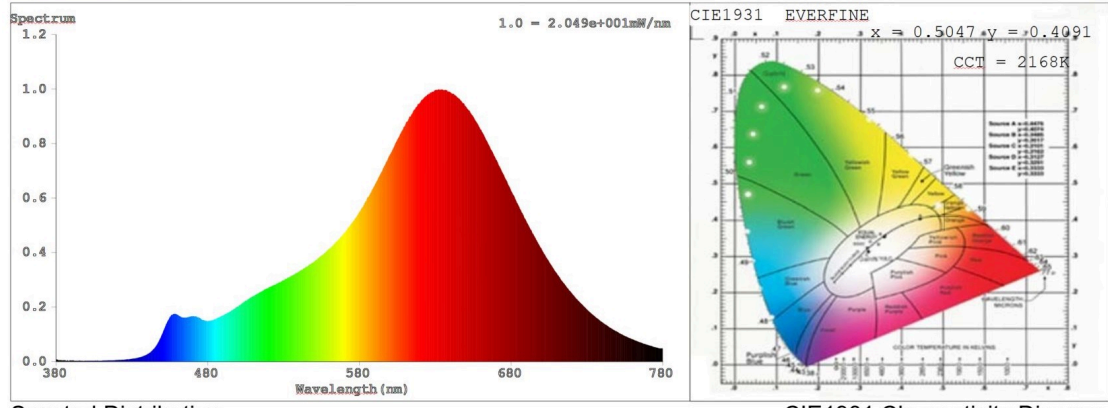
Spectral Distribution
